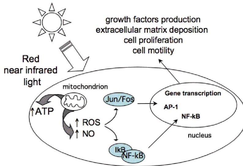
Figure 5. Cell signaling pathways induced by LLLT.
